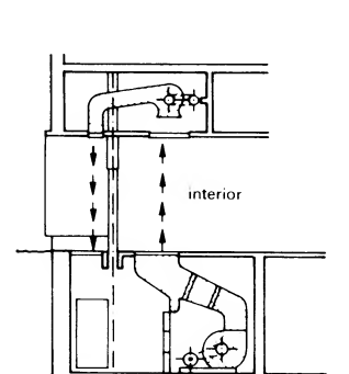
19 Air curtain installation → ⑨
